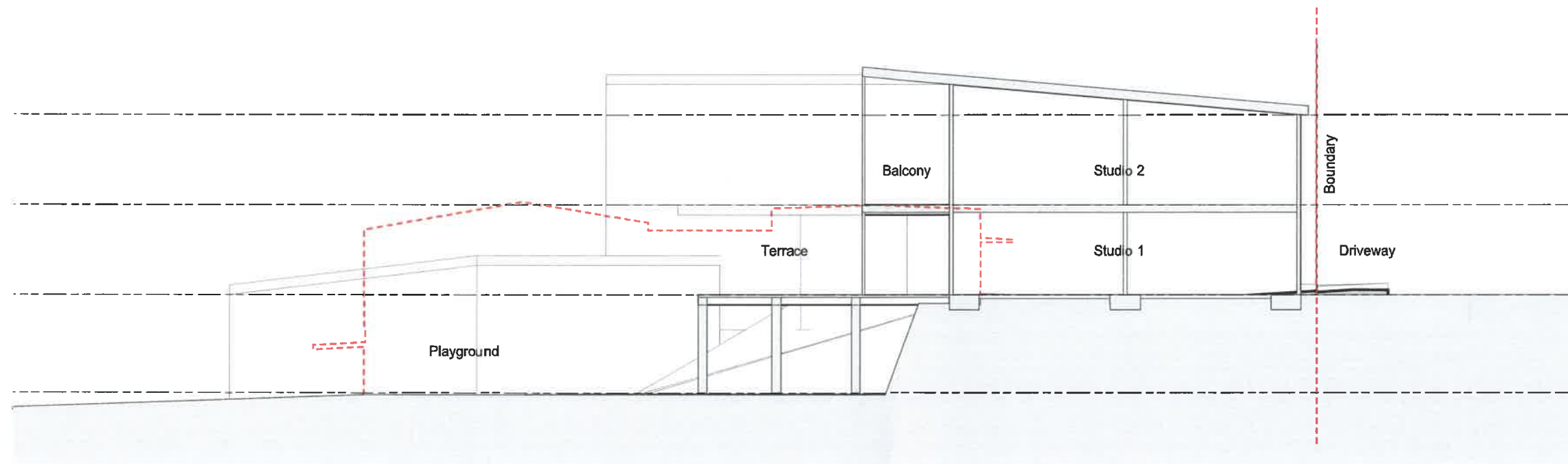
Section AA 1:200
